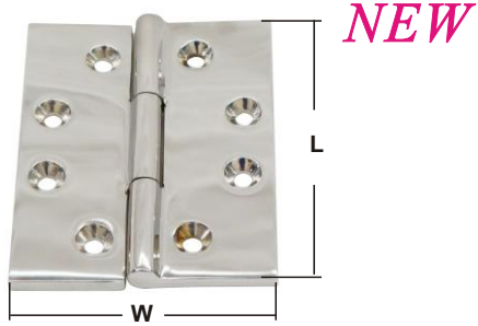
DOOR HINGE precision casted AISI 316 ITEM NO. WxLmm Thickness Weight/g 008515 80x100(3-3/16"x4") 4mm 300
