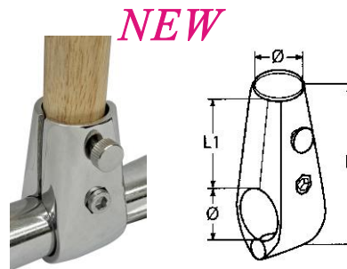
NEW RAIL MOUNT FLAG POLE SOCKET casted AISI 316 ITEM NO. for tube- \Phi L L1 B22-004 25mm 20mm 40mm
