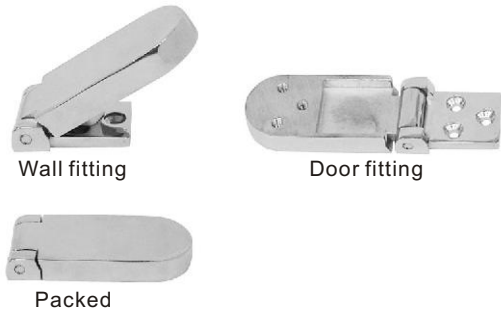
HEAVY DUTY HINGE casted AISI 316 Packed Wall fitting Door fitting ITEM NO. mm mm mm Weight/g 008614 45x30 25x30 20x30 92
