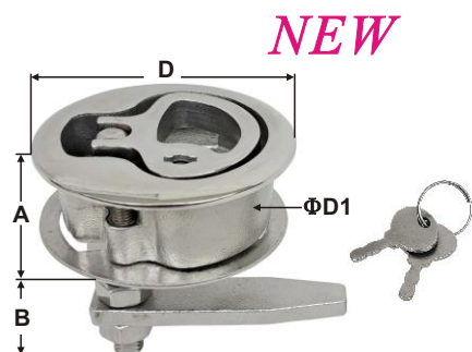
LIFTING HANDLE WITH KEY AISI 316
