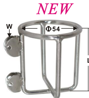
BOAT HOOK HOLDER AISI 304 ITEM NO. L mm Φ mm W mm B19-044 79 54 up to 7mm wire
