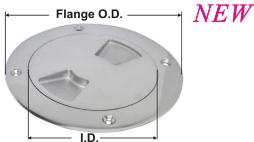
INSPECTION PORT casted AISI 316
