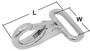
CARBINE HOOK AISI 316 ITEM NO. L mm W mm Weight/g 000407 50(2") 25(1") 25
