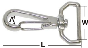
WEB SWIVEL SNAP HOOK Casted AISI 316 ITEM NO. Amm Lmm Wmm Weight/g 000411 9 65 28 30
