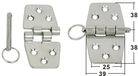
HINGE WITH PIN stamped AISI 304 ITEM NO. Thickness Weight/g 008514 2mm 50
