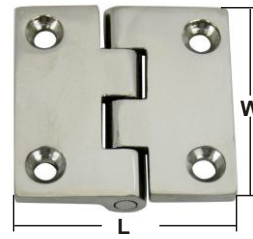
DOOR HINGE precision casted AISI 316 Reverse ITEM NO. WxLmm Thickness Weight/g 008511 50x50(2"x2") 4.5mm 89
