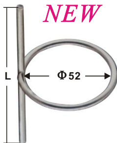
BOAT HOOK HOLDER AISI 304 Simple fixing e. g. with tap, clamp ITEM NO. L mm L1 mm Φ mm B19-041 102 60 52
