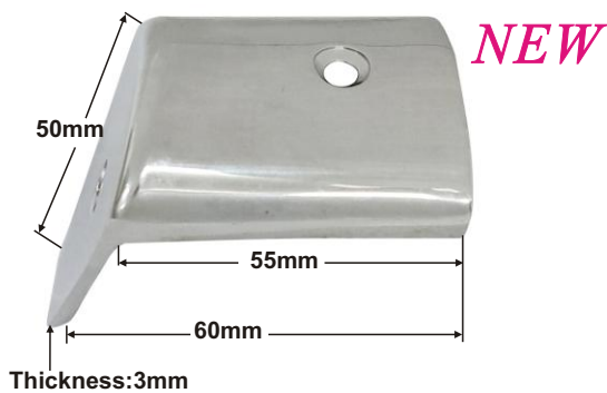
FENDER STRIP AISI 316 To mount on support PVC UV bases ITEM NO. B23-024
