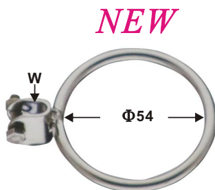
BOLDING RING FOR BOAT HOOK AISI 304 ITEM NO. Φ mm W mm B19-043 54 up to 7mm wire
