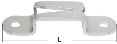
V CLEAT AISI 304 For school masts and booms ITEM NO. L mm 008703 50
