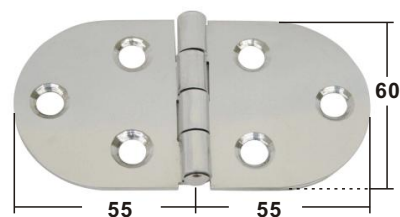
HINGE stamped AISI 304 ITEM NO. Thickness Weight/g 008513 2mm 95
