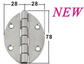
HINGE stamped AISI 304 ITEM NO. Thickness Weight/g B19-028 2mm 70
