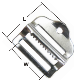
BUCKLE AISI 316 ITEM NO. L mm W mm Weight/g 004323 34(1-5/16") 25(1") 10
