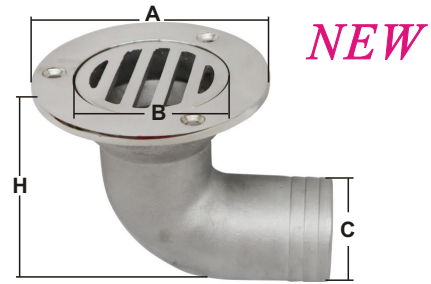
SHOW / COCKPIT DRAINERS stainless steel AISI 316 ITEM NO. Flange \Phi (A) Application hole (B) Hose adaptor (C) H mm Weight/g B19-018 80 mm 50 mm 38 mm 70 380
