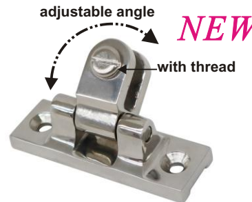
UNIVERSAL DECK HINGE casted AISI 316 ITEM NO. Base Weight/g B19-009 62x21mm(2-5/8"x1-1/8") 100
