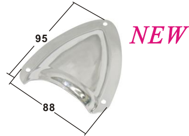
VENT AISI 304 ITEM NO. LxWxHmm Type Weight/g 003751 95x88x24 midget 50
