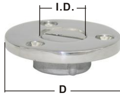
GARBOARD DRAIN PLUG casted AISI 316 ITEM NO. I.D D Weight 003781 17mm 50mm(2") 90g
