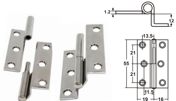
LIFT OFF HINGE stamped AISI 304 ITEM NO. Note Weight/g B18-015L Right handed 36 B18-015R Left handed 36
