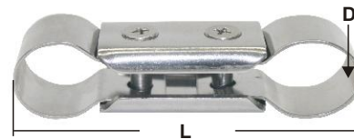
GRAB HANDLE CONNECTION stamped AISI 316 ITEM NO. L mm D mm Weight/g 009656 90(3-1/2") 22(7/8") 009664 90(3-1/2") 25(1")
