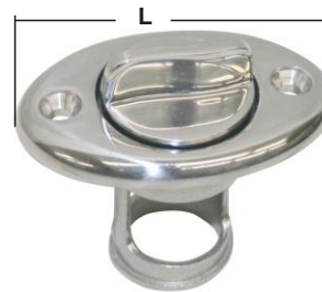
GARBOARD DRAIN PLUG casted AISI 316 Thread, removeable plug highly polished. ITEM NO. Hole mm L mm Weight/g 003780 27(1") 64(2-9/16") 110
